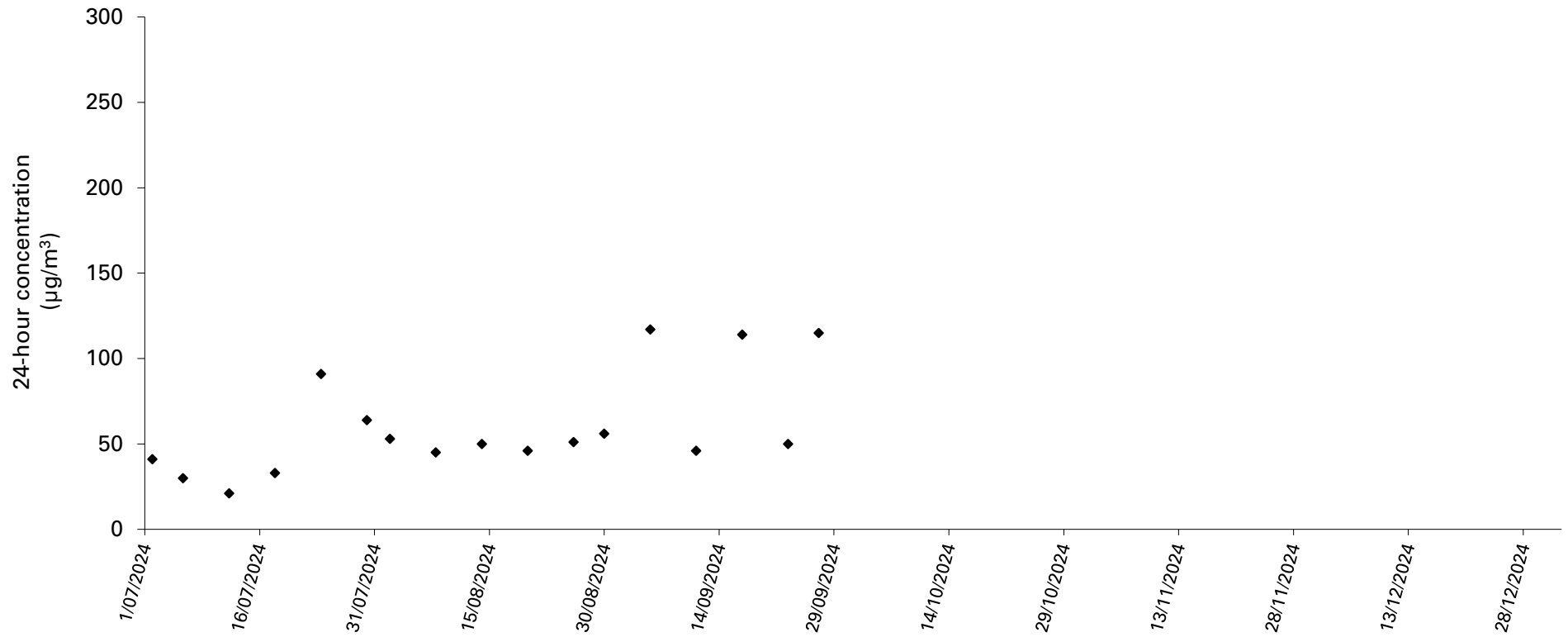
24-hour TSP concentration vs date for Location W-A6
